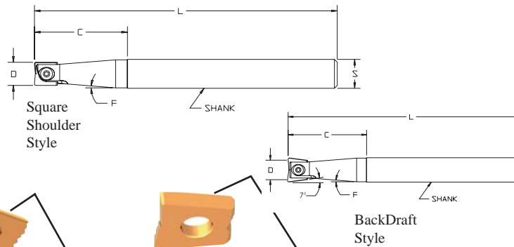
"T" Type Shank
